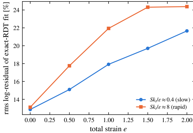
Figure 11. Scale-resolved distance between the strained ODT line spectra and exact linear theory: rms log-residual of the two-parameter exact-RDT-distorted von Kármán fit, against total strain, for slow and rapid onset strain-rate parameters (medians over 1024 realisations; identical precursor state at e = 0 ).
