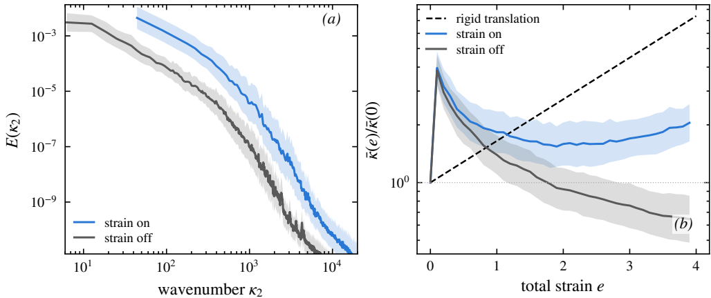
Figure 8. Full model against the matched no-strain baseline at \nu = 10^{-5} (ensemble means over 128 realisations, geometric \pm\sigma bands). (a) Final-strain total spectrum E(k_2) : the full model (strain on) extends to higher wavenumber than the baseline (strain off) but remains broadband, not a rigid translation. (b) Centroid migration: the baseline relaxes below unity, the full model is lifted above it by the compression, yet stays far below the rigid-translation line (dashed). The gap between the two solid curves is the distortion attributable to the mean strain at this Reynolds number.
