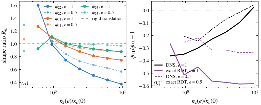
Figure 6. Exact linear theory does not translate the projected spectra rigidly. Left: shape ratio R_{nn}(\kappa_2) of the exactly distorted, line-projected component spectra to a rigid translation, at e = 1 under plane strain (closed-form Cauchy solution, isotropic initial fields, four realisations). Right: the transverse splitting \phi_{11}/\phi_{33} - 1 versus wavenumber in exact linear theory and in the strained-box DNS of § 4.2.
