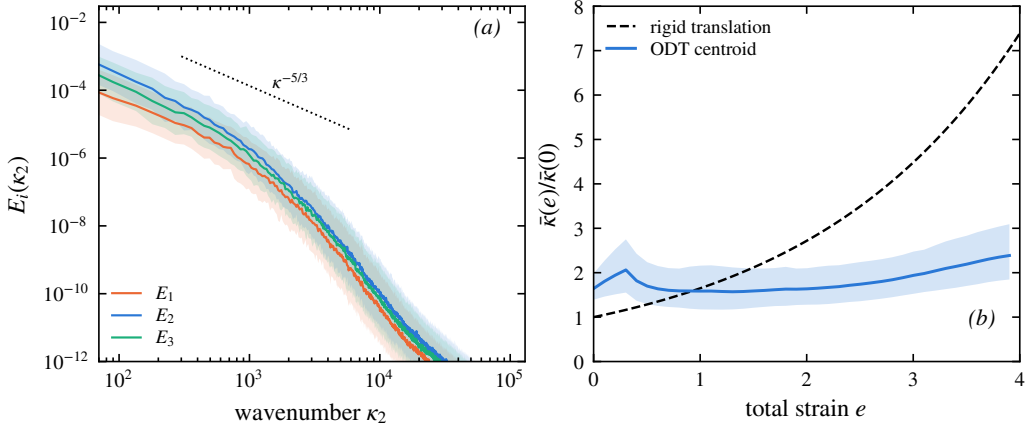
Figure 9. The physical operating point ( \nu \approx 3 \times 10^{-6} , Re_{\mathcal{L}} \approx 4.4 \times 10^3 , 16000 cells; ensemble over 200 realisations, geometric \pm\sigma ). (a) Final-strain component spectra: smooth rolloff with no grid-scale shelf; the upwash E_2 amplified above the streamwise E_1 ; dotted reference slope \kappa^{-5/3} . (b) Total-spectrum centroid migration against the rigid-translation law (dashed): the broadband distortion that linear theory cannot represent, at the operating point and with the noise averaged out.
