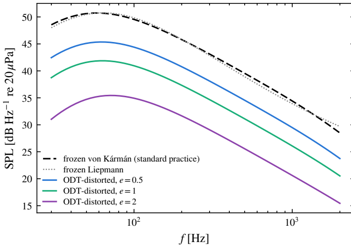
Figure 17. The assembled absolute prediction at the reference configuration of § 4.0.4: far-field sound pressure level from the compact lift-dipole form of Amiet (1975) with the exact Sears response, for a flat plate of chord 0.39 m ( Re_c \approx 5 \times 10^5 ) and span 0.8 m at U_\infty = 20 \text{ m s}^{-1} , u'/U_\infty = 6\% , \mathcal{L} = 55 \text{ mm} , observer 1 m overhead. Dashed: the frozen von Kármán inflow of standard practice (the e = 0 member of the fitted representation, which is exactly the isotropic von Kármán spectrum); grey dotted: the frozen Liepmann spectrum at the same (u', \mathcal{L}) , an independent analytic cross-check of the physical-unit bridge. Solid: the same chain with the computed distorted inflow at total strains e = 0.5, 1 and 2 ( Sk_t/\varepsilon \approx 0.4 ), level and shape both included.
