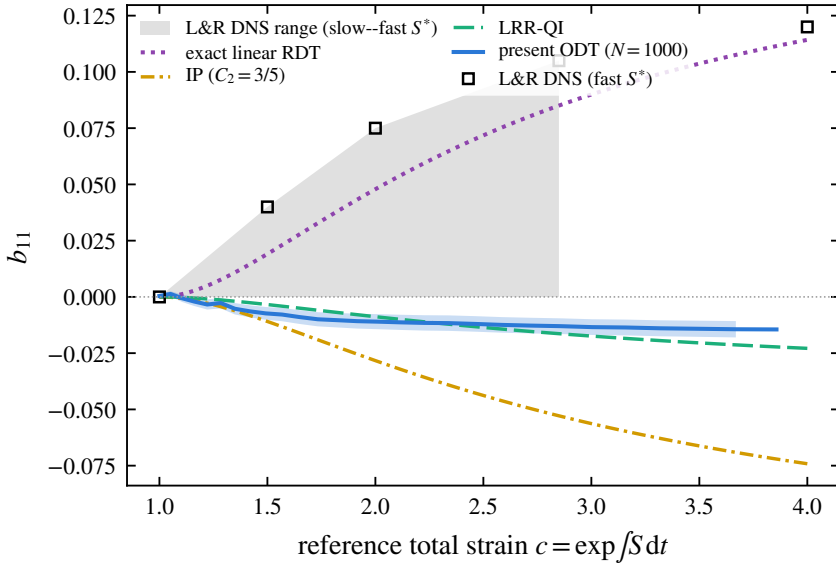
Figure 5. The unstrained-direction anisotropy b_{11} under plane strain: present model (solid, 1000 realisations, standard-error band) against exact linear rapid distortion (dotted, wavevector-ensemble integration), the IP and LRR-QI closures, and the DNS of Lee & Reynolds (1985) (symbols and shaded S^* range). The fast-strain DNS tracks exact RDT, whose rapid pressure–strain feeds the neutral direction; the single-point closures—and the model built on them—miss this orientation-carried redistribution, the deficiency measured and localised in § 5.6.
