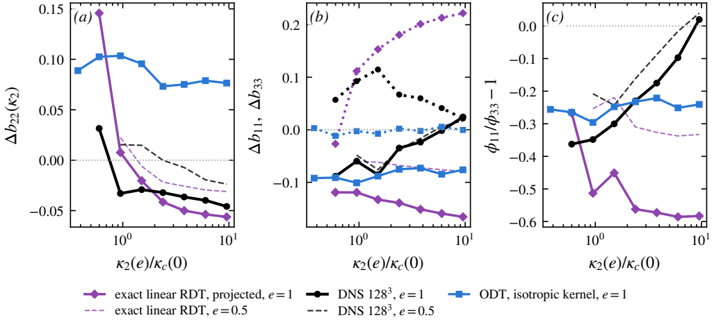
Figure 10. Three-way comparison at Sk_t/\varepsilon = 0.8 : strain-induced anisotropy of the line spectra relative to each system's own unstrained state; strain-coupled ODT (1024 realisations) against exact projected RDT and DNS ( 128^3 , four realisations); e = 1 solid, e = 0.5 dashed.
